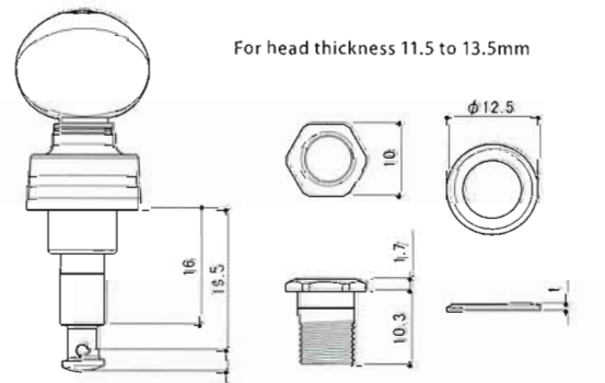
Aluminum Button
