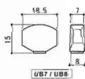
Plastic Button
